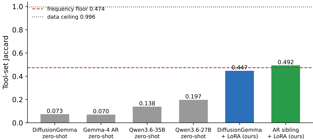
Held-out tool selection: fine-tunes vs. zero-shot, floor, and ceiling
