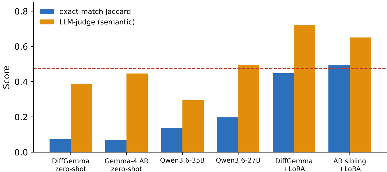
The dialect tax: exact-match understates models 5-6x
