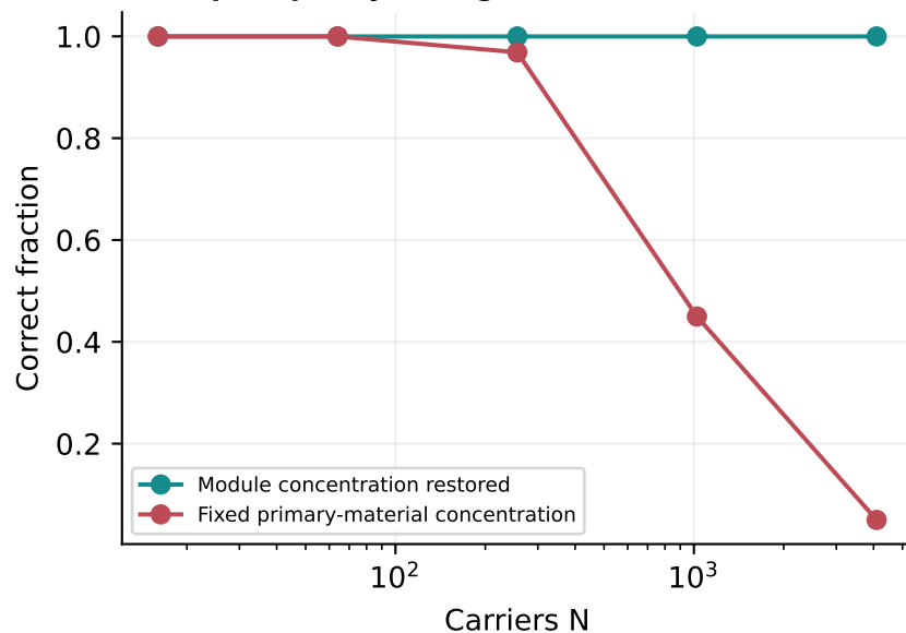
Conditional threshold recurrence, C = 28
