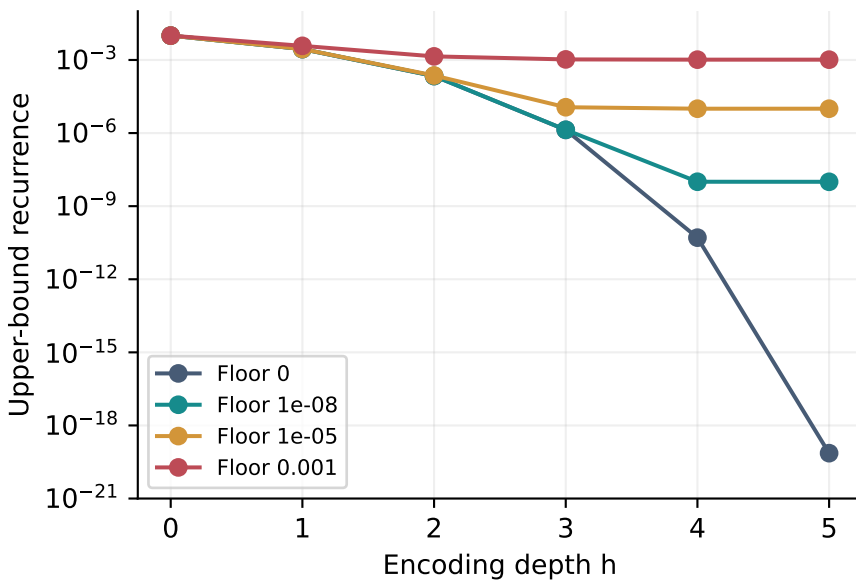
Conditional threshold recurrence, C = 28
