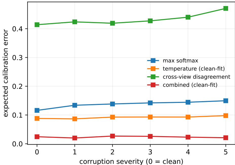
Calibration degrades with corruption
